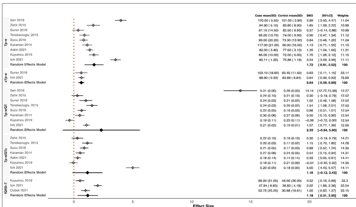
Figure 4: Forest plots showing the standardized mean differences (SMDs) of T-peak to T-end (Tp-e) and its division on QT and corrected QT intervals and frontal QRS-T angle using the random-effect model between Coronary Slow Flow Phenomenon (CSFP) and control groups. Heterogeneity ( I^2 ): Tp-e: 96.43%, cTp-e: 0%, Tp-e/QT: 98.24%, Tp-e/QTc: 97.62%, fragmented QRS (fQRS)-T: 94.52%. CI: confidence interval; SD: standard deviation; QTc: Corrected QT interval.
